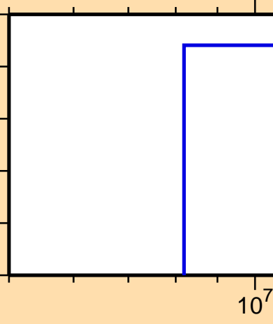
\sigma vs. E for ^{154}\text{Ho} (mt 42)
