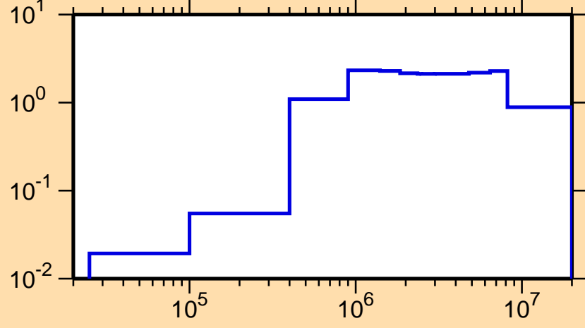
\sigma vs. E for ^{154}\text{Ho}(n,\text{inel.})
