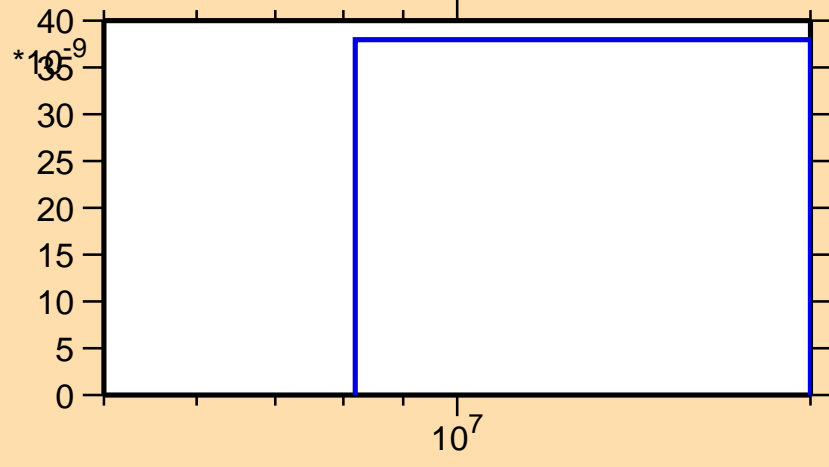
\sigma vs. E for ^{154}\text{Ho}(n,\text{nt})
