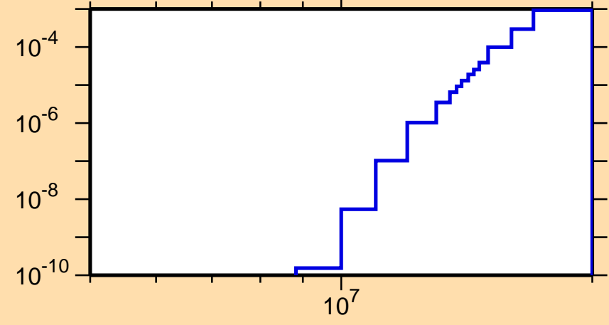
\sigma vs. E for ^{154}\text{Ho}(n,2n\alpha)
