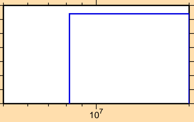
\sigma vs. E for ^{154}\text{Ho} (mt 34)
