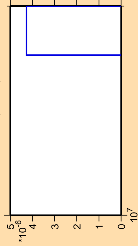
\Delta\sigma/\sigma vs. E for ^{155}\text{Ho} (mt 42)
