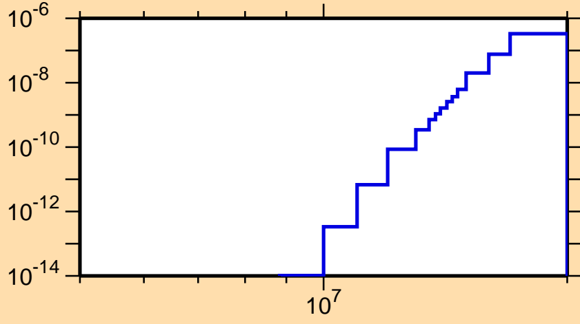
\sigma vs. E for ^{155}\text{Ho} (mt 45)
