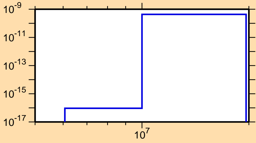
\sigma vs. E for ^{155}\text{Ho}(\text{mt117})
