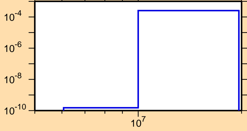
\sigma vs. E for ^{155}\text{Ho}(n,t)
