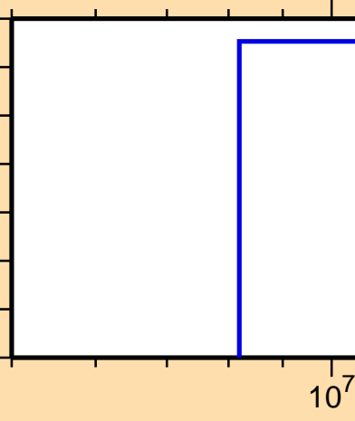
\sigma vs. E for ^{155}\text{Ho} (mt 34)
