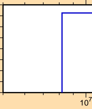
\sigma vs. E for ^{155}\text{Ho} (mt 42)
