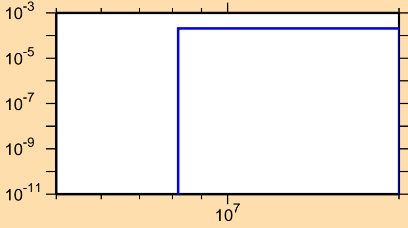
\sigma vs. E for ^{155}\text{Ho}(n,t)
