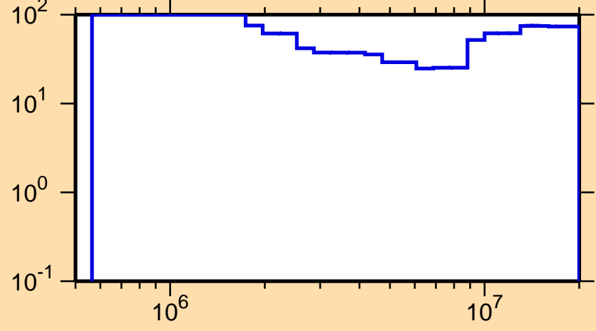
\Delta\sigma/\sigma vs. E for ^{156}\text{Ho}(n,n\text{cont.})
