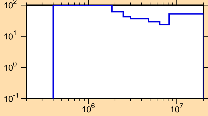
\Delta\sigma/\sigma vs. E for ^{156}\text{Ho}(n,ncont.)
