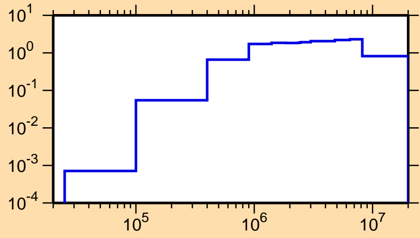
\sigma vs. E for ^{156}\text{Ho}(n,\text{inel.})
