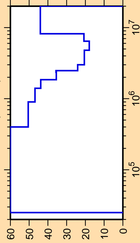
\Delta\sigma/\sigma vs. E for ^{156}\text{Ho}(n,\text{inel.})
