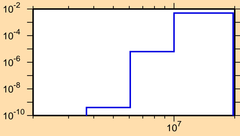
\sigma vs. E for ^{156}\text{Ho}(n,d)
