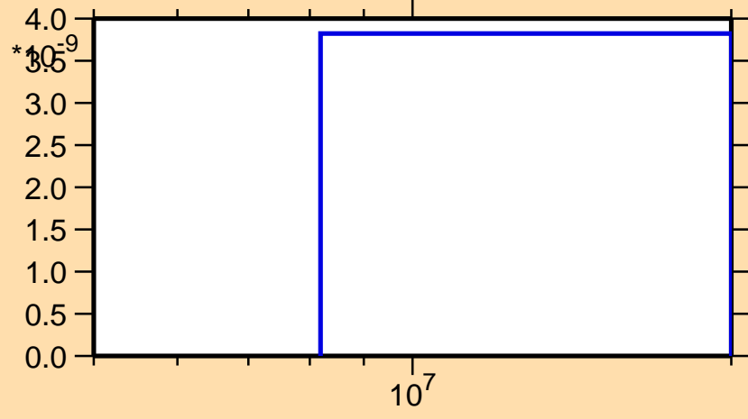
\sigma vs. E for ^{156}\text{Ho}(\text{mt } 45)
