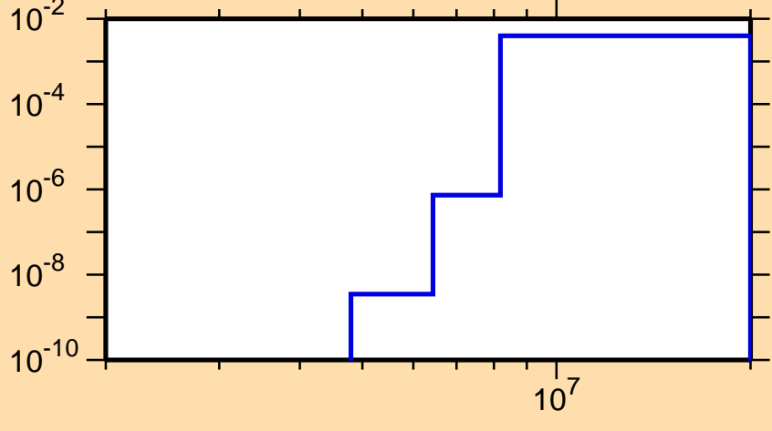
\sigma vs. E for ^{156}\text{Ho}(n,d)
