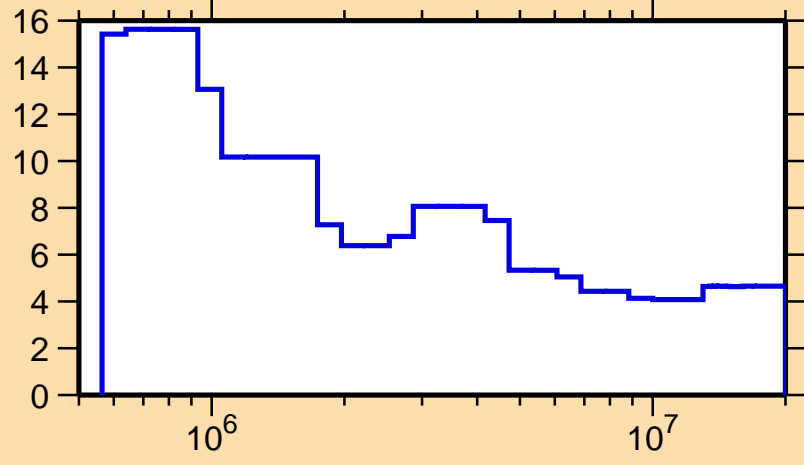
\Delta\sigma/\sigma vs. E for ^{157}\text{Ho}(n,n\text{onel.})
