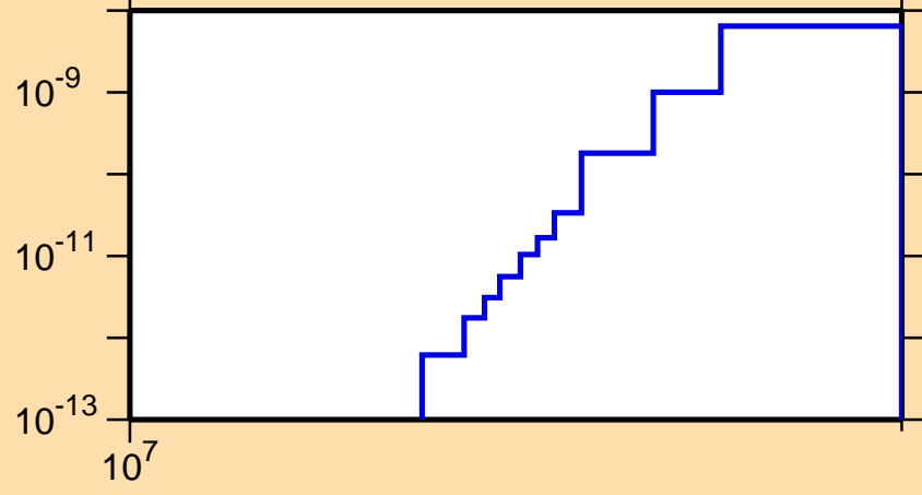
\sigma vs. E for ^{157}\text{Ho} (mt 45)
