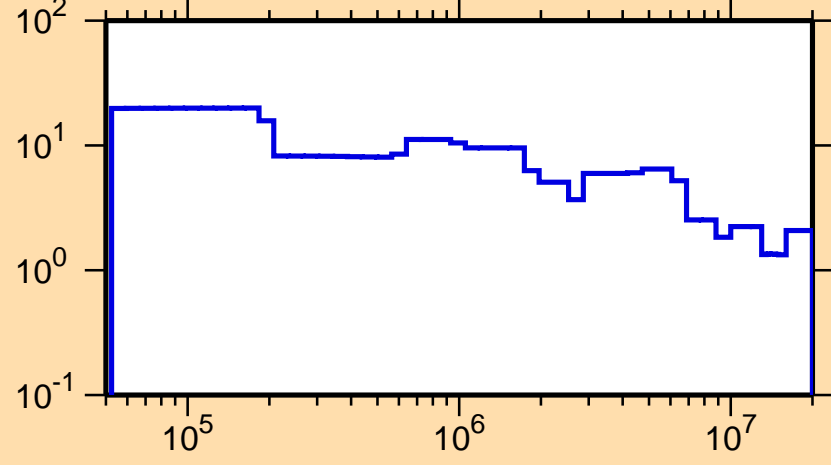
\Delta\sigma/\sigma vs. E for ^{157}\text{Ho}(n,\text{tot.})
