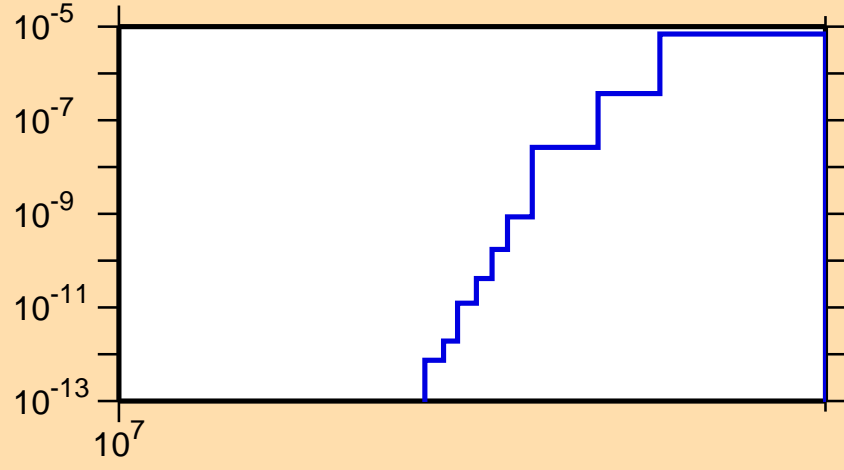
\sigma vs. E for ^{157}\text{Ho}(n,\text{nd})
