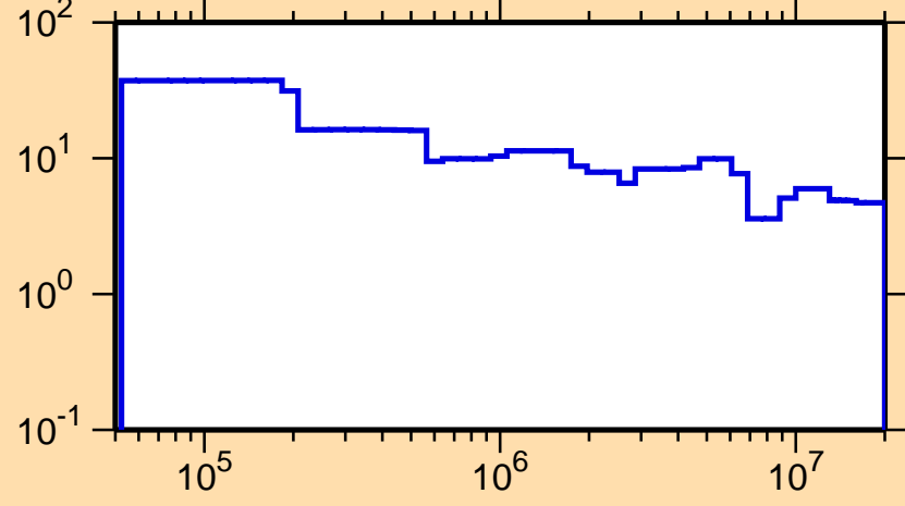
\Delta\sigma/\sigma vs. E for ^{157}\text{Ho}(n,\text{el.})
