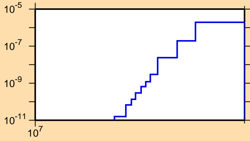
\sigma vs. E for ^{157}\text{Ho}(n,2n\alpha)
