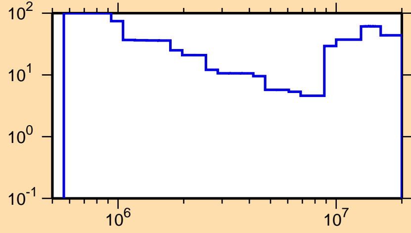
\Delta\sigma/\sigma vs. E for ^{157}\text{Ho}(n,ncont.)
