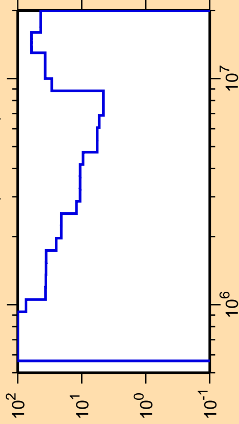
\Delta\sigma/\sigma vs. E for ^{157}\text{Ho}(n,n_{\text{cont}}) .
