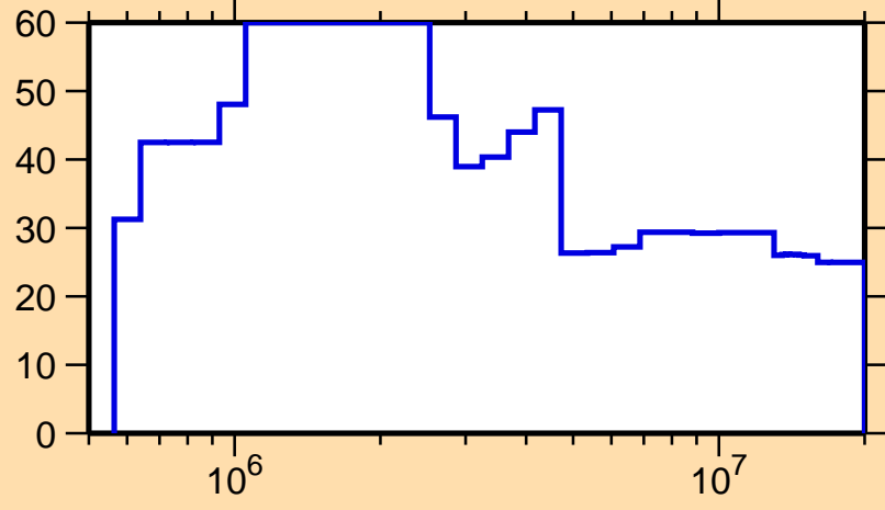
\Delta\sigma/\sigma vs. E for ^{157}\text{Ho}(n,n_1)
