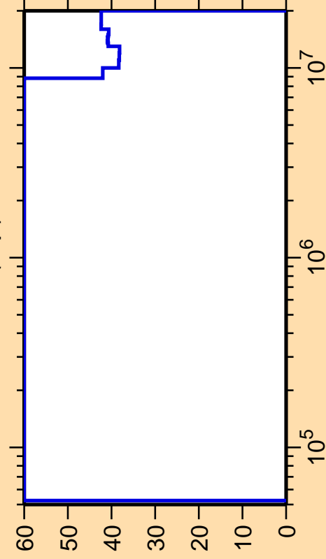
\Delta\sigma/\sigma vs. E for ^{157}\text{Ho}(n,p)
