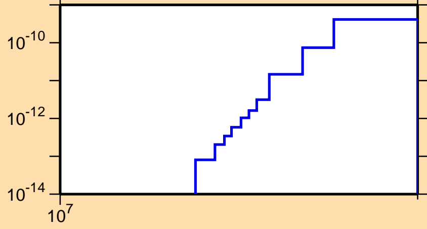
\sigma vs. E for ^{157}\text{Ho}(\text{mt117})
