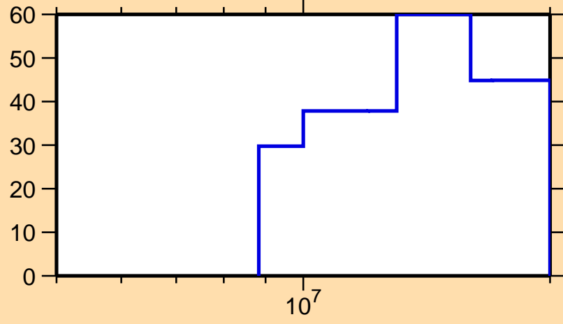
\Delta\sigma/\sigma vs. E for ^{157}\text{Ho}(n,\text{inel.})
