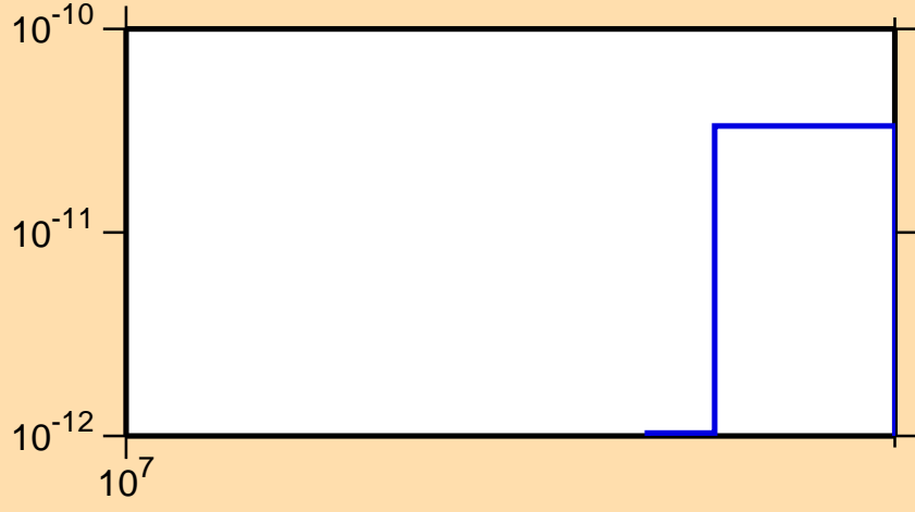
\sigma vs. E for ^{157}\text{Ho}(n,\text{pd})
