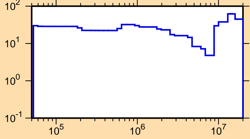
\Delta\sigma/\sigma vs. E for ^{157}\text{Ho}(n,\text{inel.})
