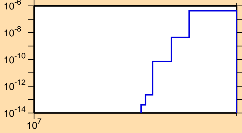
\sigma vs. E for ^{157}\text{Ho}(n,nt)
