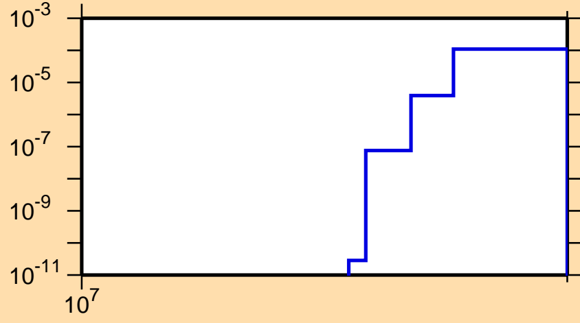
\sigma vs. E for ^{157}\text{Ho}(n,2np)
