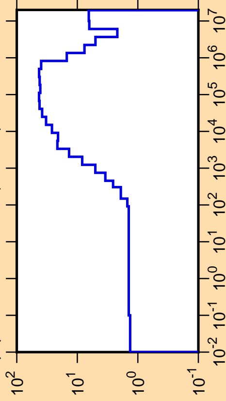
\Delta\mu/\mu vs. E for ^{157}\text{Ho}(\text{mt251})
