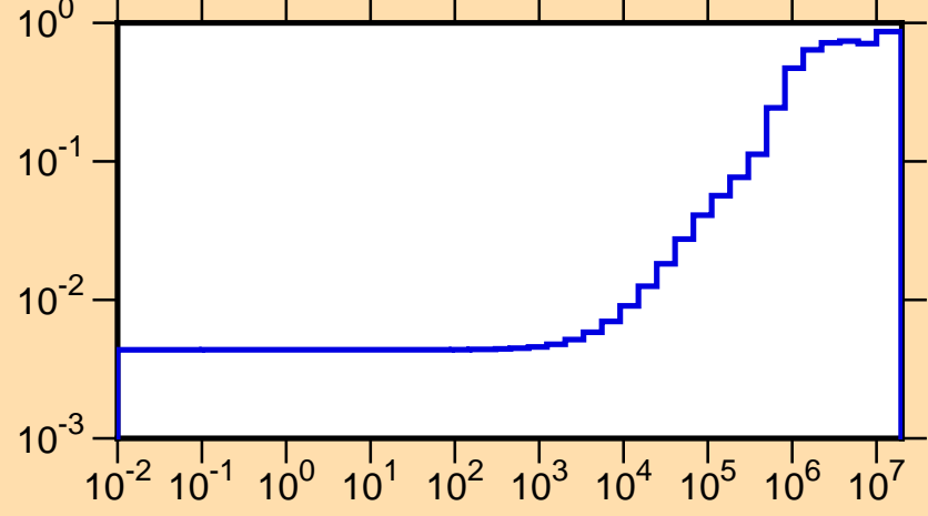
\mu vs. E for ^{157}\text{Ho}(\text{mt251})
