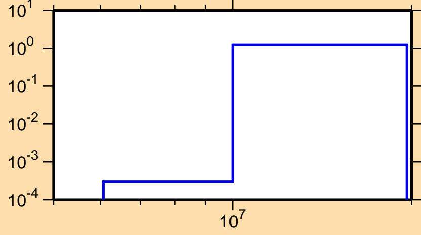
\sigma vs. E for ^{157}\text{Ho}(n,2n)
