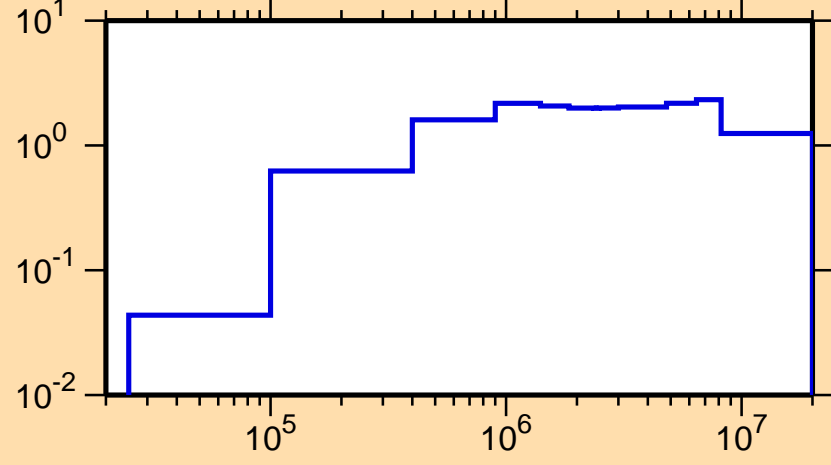
\sigma vs. E for ^{157}\text{Ho}(n,\text{inel.})
