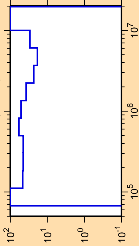
\Delta\sigma/\sigma vs. E for ^{158}\text{Ho}(n,\text{inel.})
