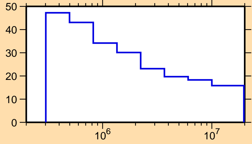
\Delta\sigma/\sigma vs. E for ^{158}\text{Ho}(n,n\text{onel.})
