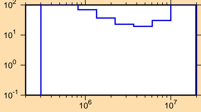
\Delta\sigma/\sigma vs. E for ^{158}\text{Ho}(n,ncont.)
