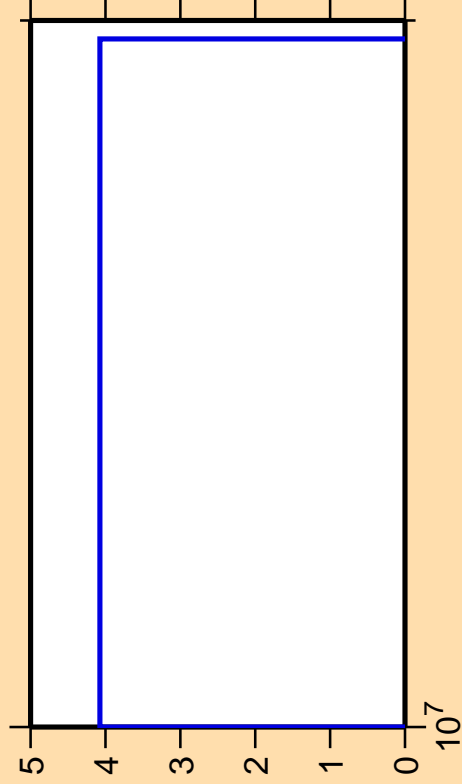
\Delta\sigma/\sigma vs. E for ^{158}\text{Ho}(\text{mt117})
