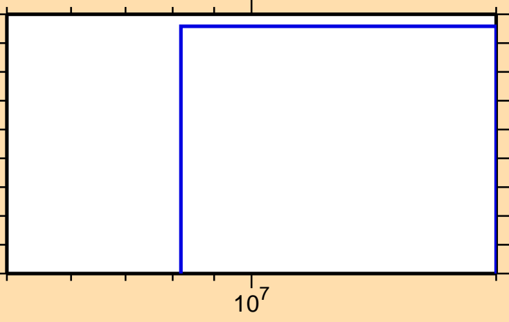
\sigma vs. E for ^{158}\text{Ho}(n,\text{nd})
