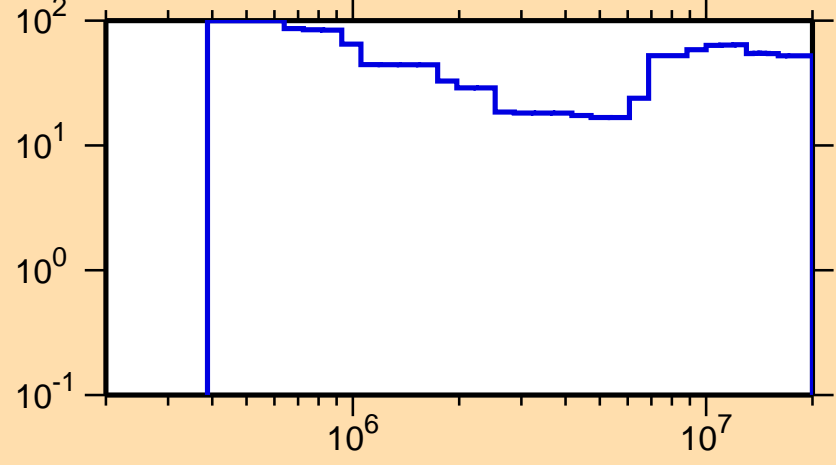
\Delta\sigma/\sigma vs. E for ^{158}\text{Ho}(n,n\text{cont.})
