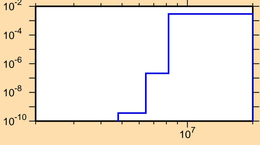
\sigma vs. E for ^{158}\text{Ho}(n,d)
