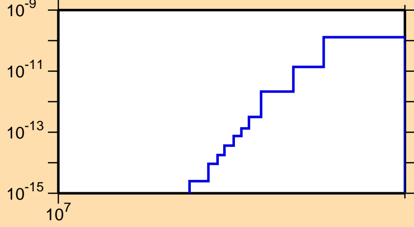
\sigma vs. E for ^{158}\text{Ho}(\text{mt } 45)
