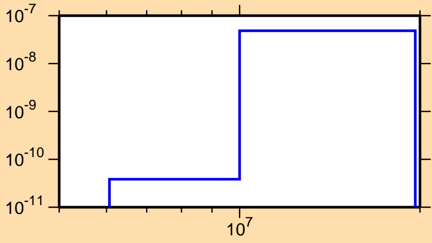
\sigma vs. E for ^{158}\text{Ho}(n,p\alpha)
