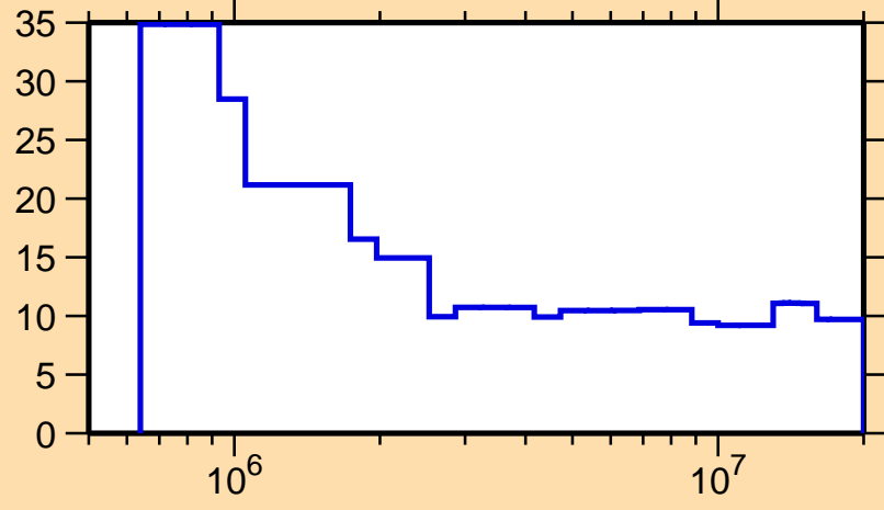
\Delta\sigma/\sigma vs. E for ^{159}\text{Ho}(n,n\text{onel.})
