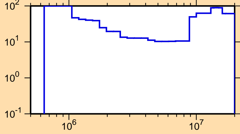
\Delta\sigma/\sigma vs. E for ^{159}\text{Ho}(n,ncont.)
