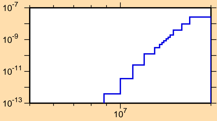
\sigma vs. E for ^{159}\text{Ho}(n,p\alpha)
