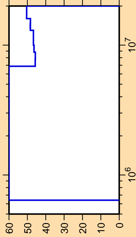
\Delta\sigma/\sigma vs. E for ^{159}\text{Ho}(n,p)
