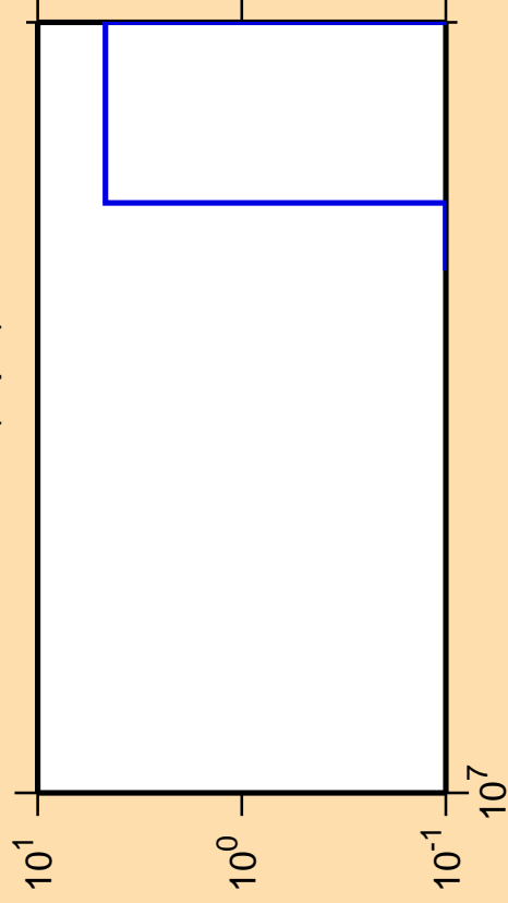
\Delta\sigma/\sigma vs. E for ^{159}\text{Ho}(n,\text{pd})
