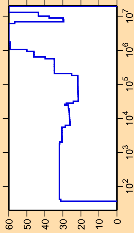
\Delta\sigma/\sigma vs. E for ^{159}\text{Ho}(n,\gamma)
