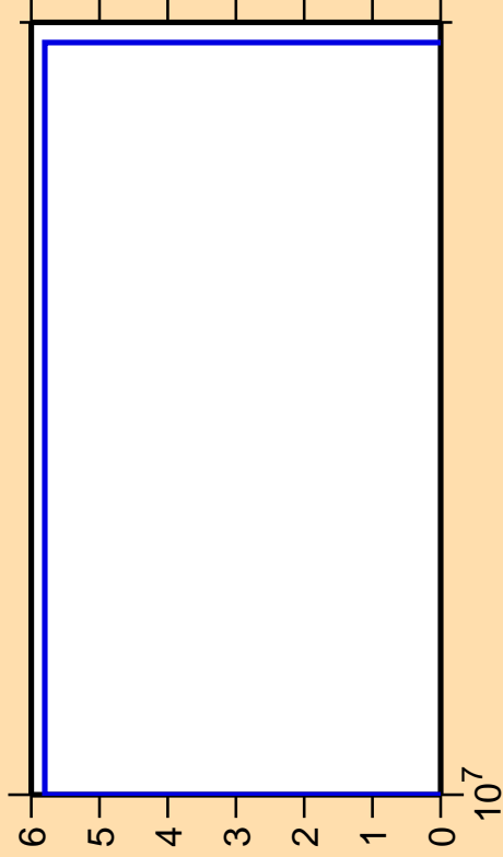
\Delta\sigma/\sigma vs. E for ^{159}\text{Ho}(\text{mt117})
