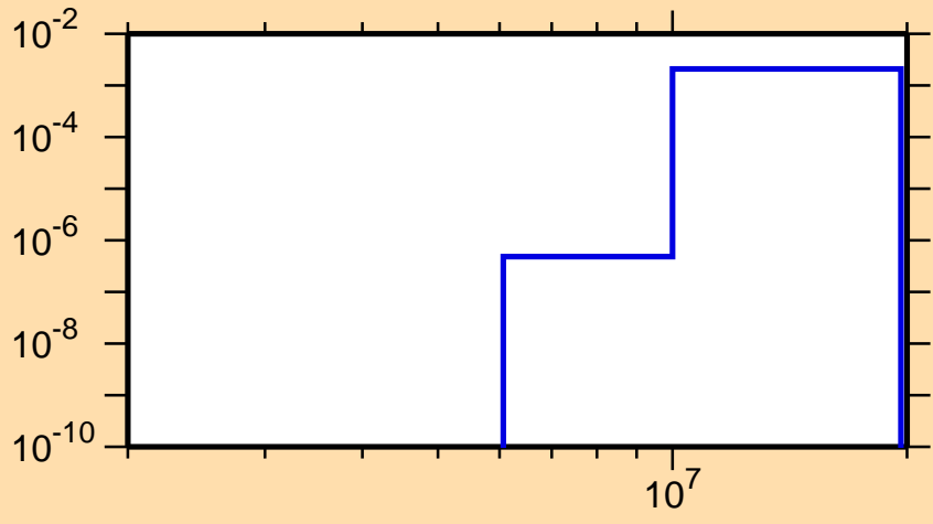
\sigma vs. E for ^{159}\text{Ho}(n,d)
