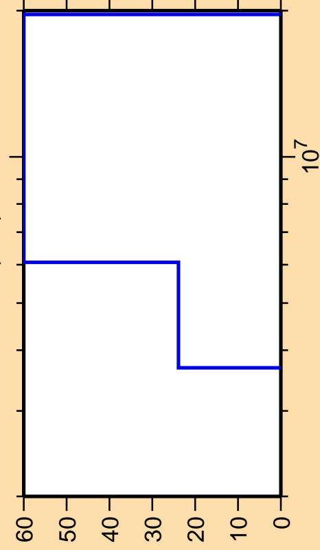
\Delta\sigma/\sigma vs. E for ^{159}\text{Ho}(n,d)
