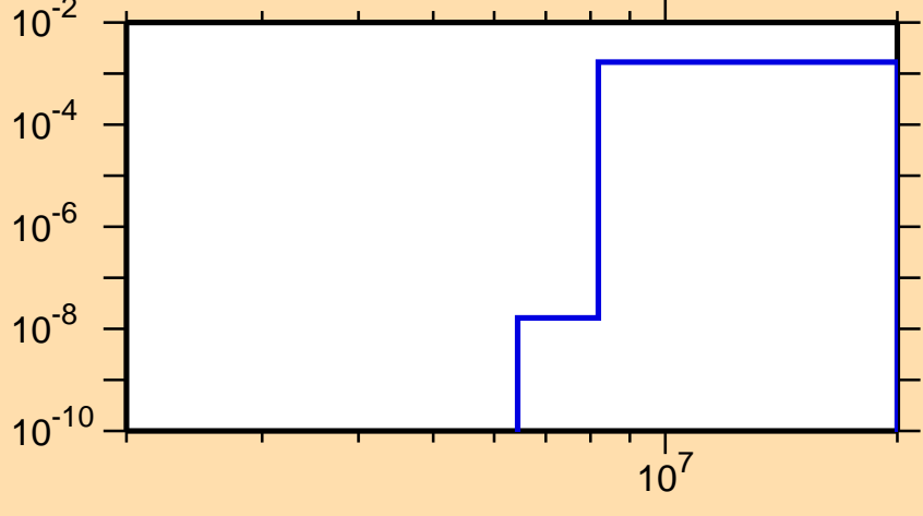
\sigma vs. E for ^{159}\text{Ho}(n,d)
