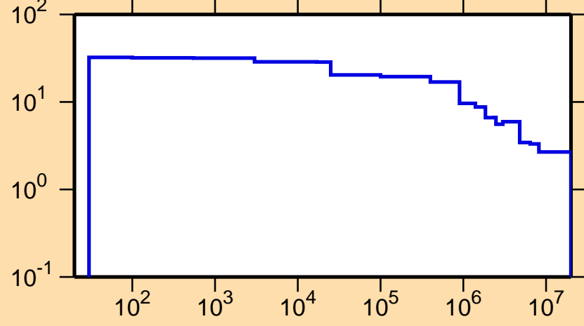
\Delta\sigma/\sigma vs. E for ^{159}\text{Ho}(n,\text{nonel.})
