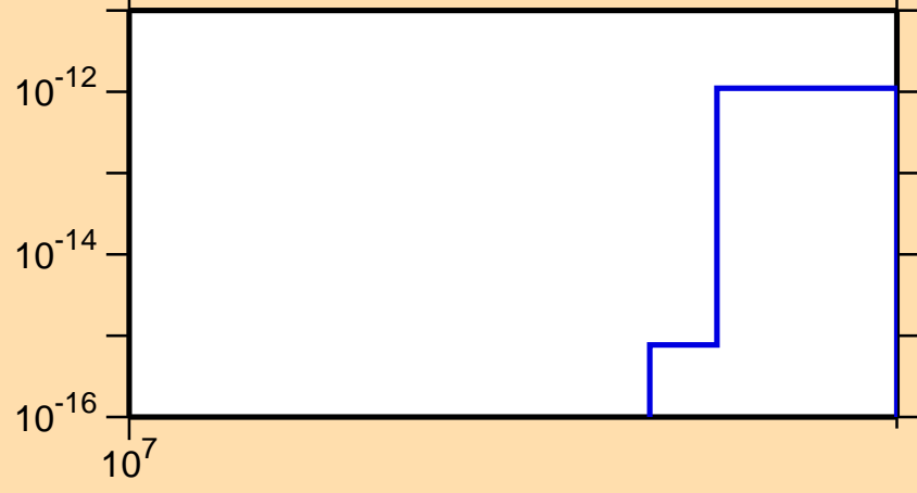
\sigma vs. E for ^{160}\text{Ho} (mt 34)
