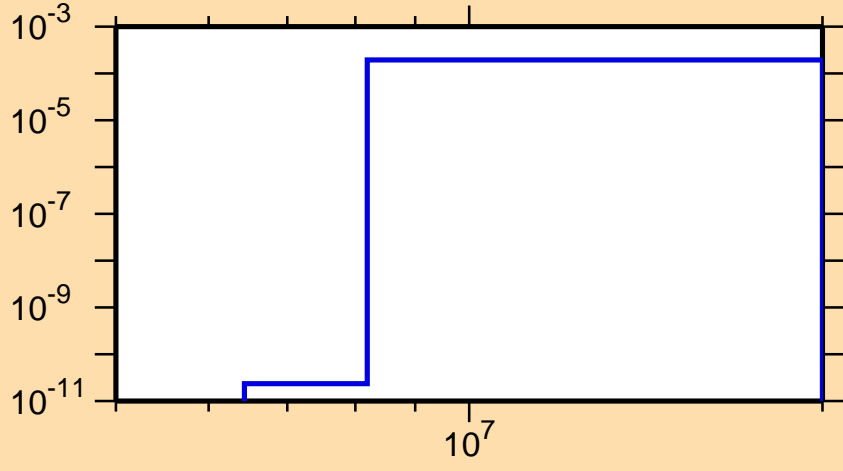
\sigma vs. E for ^{160}\text{Ho}(n,t)
