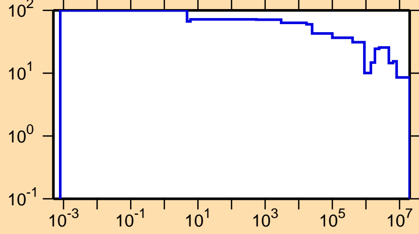
\Delta\sigma/\sigma vs. E for ^{160}\text{Ho}(n,\text{el.})
