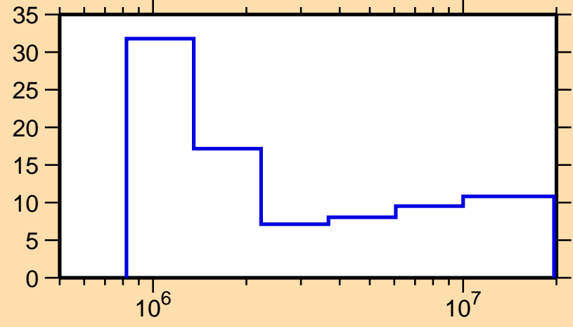
\Delta\sigma/\sigma vs. E for ^{160}\text{Ho}(n,n\text{onel.})
