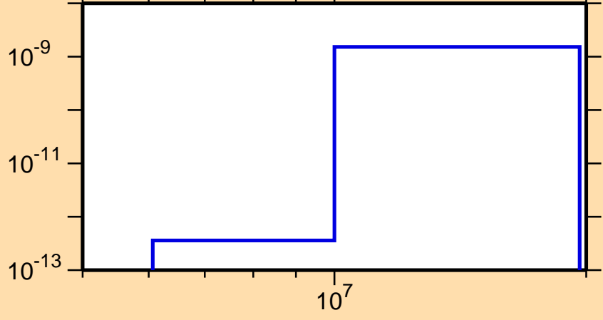
\sigma vs. E for ^{160}\text{Ho}(n,p\alpha)
