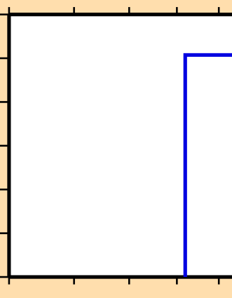
\sigma vs. E for ^{160}\text{Ho} (mt 45)
