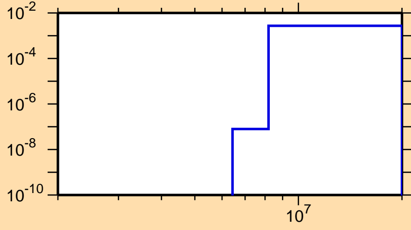
\sigma vs. E for ^{160}\text{Ho}(n,d)
