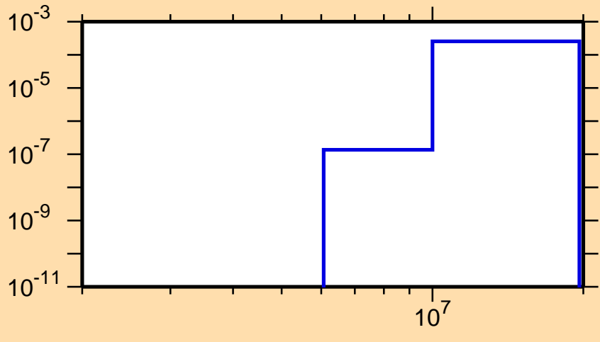
\sigma vs. E for ^{161}\text{Ho}(n,n\alpha)
