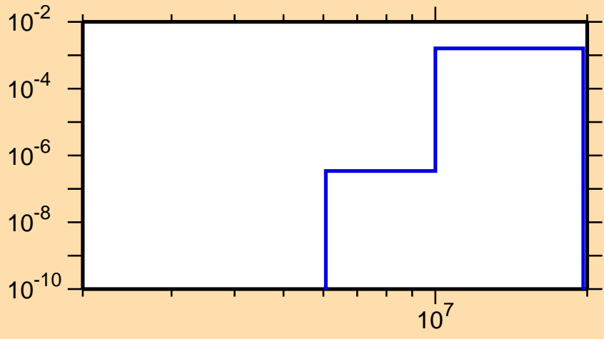
\sigma vs. E for ^{161}\text{Ho}(n,d)
