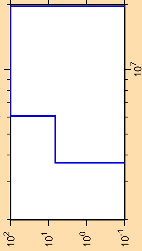
\Delta\sigma/\sigma vs. E for ^{161}\text{Ho}(n,n\alpha)
