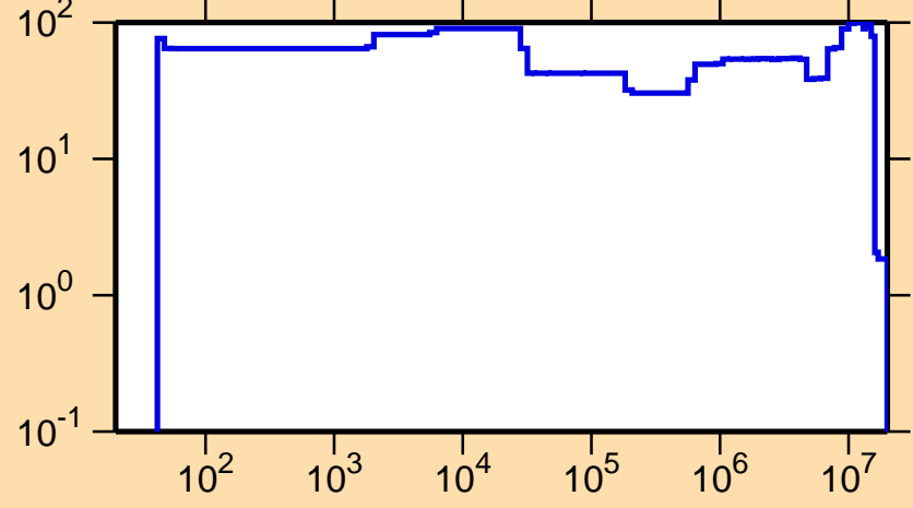
\Delta\sigma/\sigma vs. E for ^{161}\text{Ho}(n,n_1)
