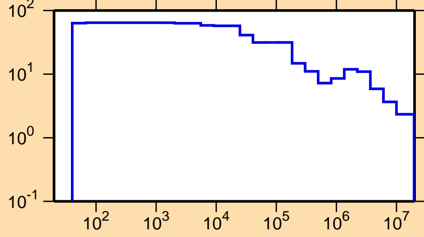
\Delta\sigma/\sigma vs. E for ^{161}\text{Ho}(n,\text{tot.})
