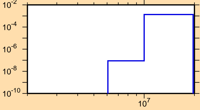
\sigma vs. E for ^{161}\text{Ho}(n,d)
