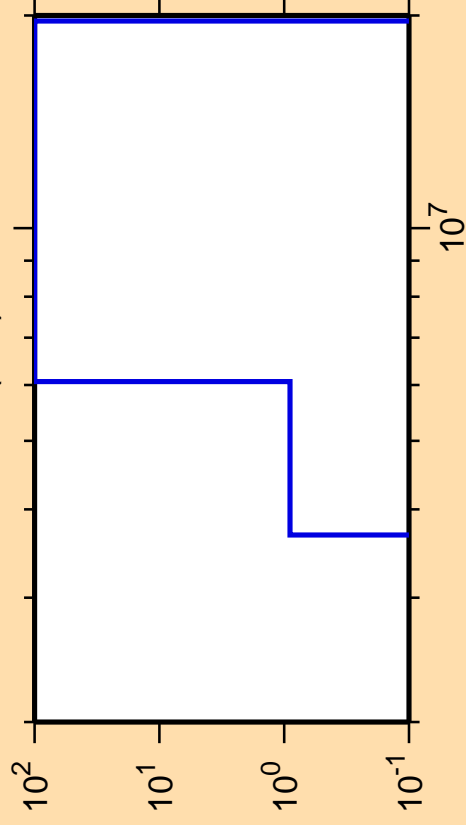
\Delta\sigma/\sigma vs. E for ^{161}\text{Ho}(n,d)
