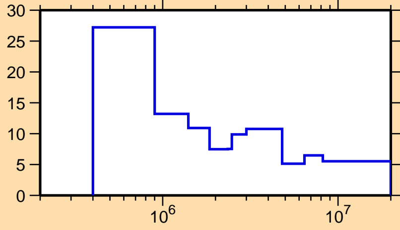
\Delta\sigma/\sigma vs. E for ^{161}\text{Ho}(n,n\text{onel.})
