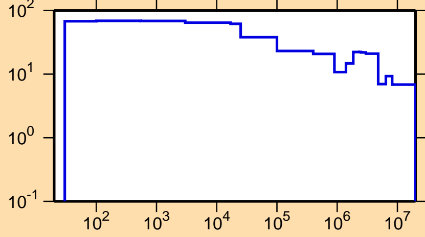
\Delta\sigma/\sigma vs. E for ^{161}\text{Ho}(n,\text{el.})
