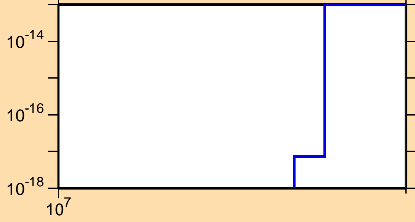
\sigma vs. E for ^{162}\text{Ho} (mt 34)
