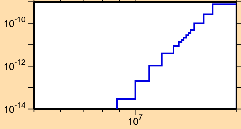
\sigma vs. E for ^{162}\text{Ho}(n,p\alpha)
