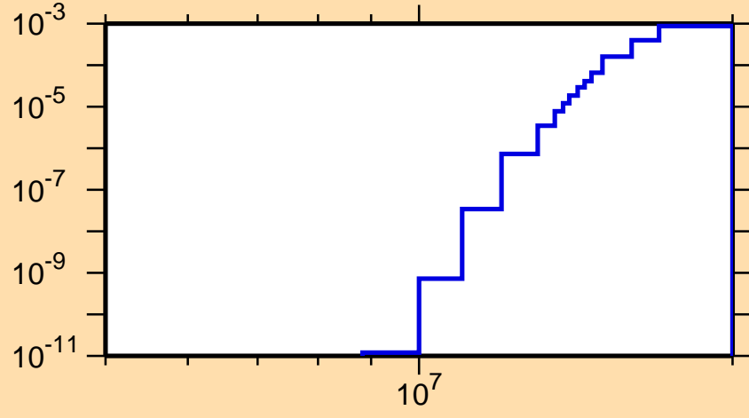
\sigma vs. E for ^{163}\text{Ho}(n,t)
