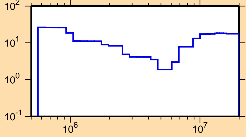
\Delta\sigma/\sigma vs. E for ^{163}\text{Ho}(n,ncont.)
