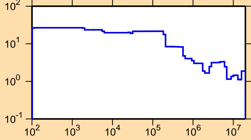
\Delta\sigma/\sigma vs. E for ^{163}\text{Ho}(n,\text{tot.})
