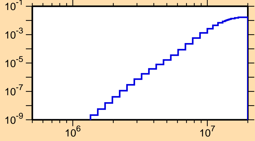
\sigma vs. E for ^{163}\text{Ho}(n,p)
