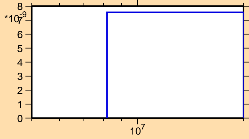
\sigma vs. E for ^{164}\text{Ho}(n,\text{nt})
