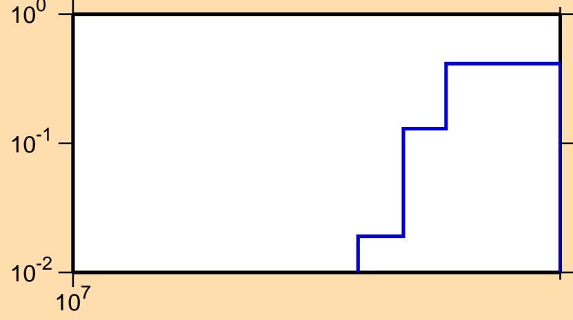
\sigma vs. E for ^{164}\text{Ho}(n,3n)
