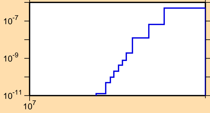
\sigma vs. E for ^{164}\text{Ho}(n,2n\alpha)
