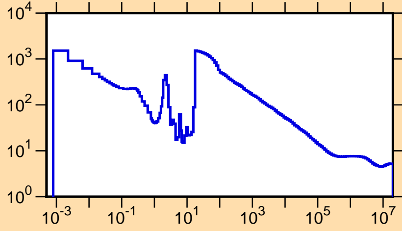
\sigma vs. E for ^{164}\text{Ho}(n,\text{tot.})
