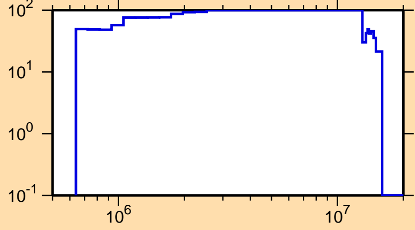
\Delta\sigma/\sigma vs. E for ^{164}\text{Ho}(n,n_1)
