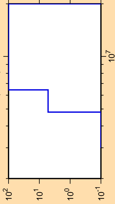
\Delta\sigma/\sigma vs. E for ^{164}\text{Ho}(n,n\alpha)
