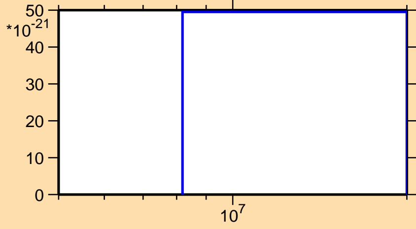
\sigma vs. E for ^{164}\text{Ho} (mt 11)
