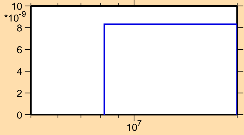
\sigma vs. E for ^{164}\text{Ho}(n,2n\alpha)
