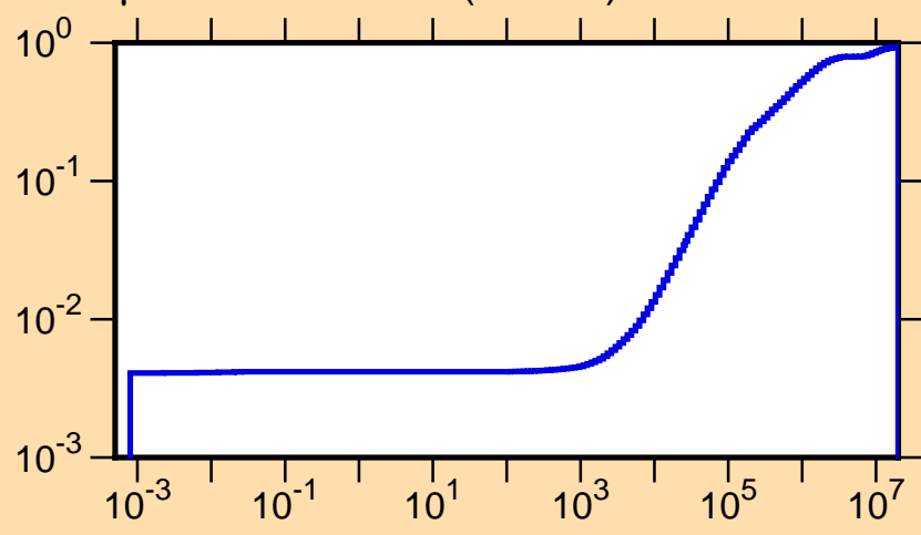
\mu vs. E for ^{165}\text{Ho}(\text{mt251})
