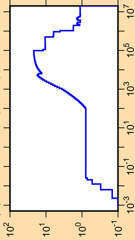
\Delta\mu/\mu vs. E for ^{165}\text{Ho}(\text{mt251})
