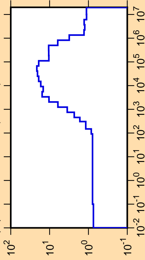
\Delta\mu/\mu vs. E for ^{165}\text{Ho}(\text{mt251})
