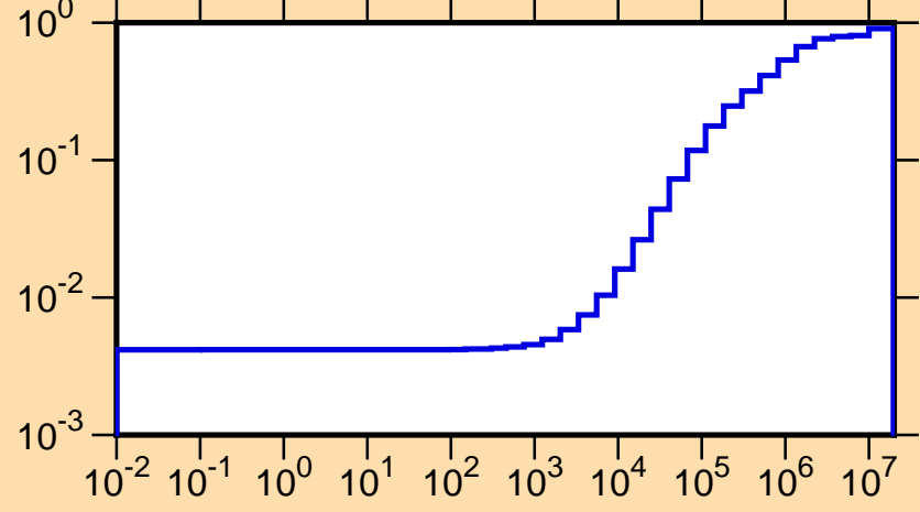
\mu vs. E for ^{165}\text{Ho}(\text{mt251})
