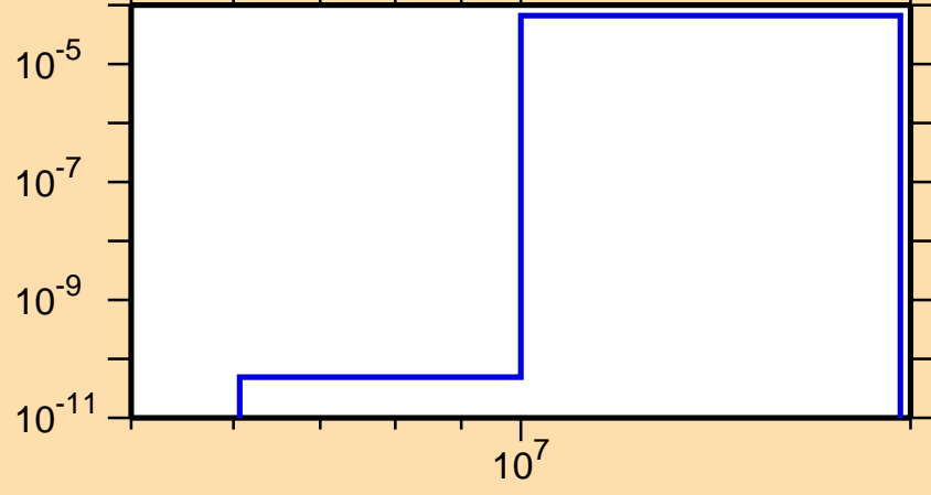
\sigma vs. E for ^{166}\text{Ho}(n,t)
