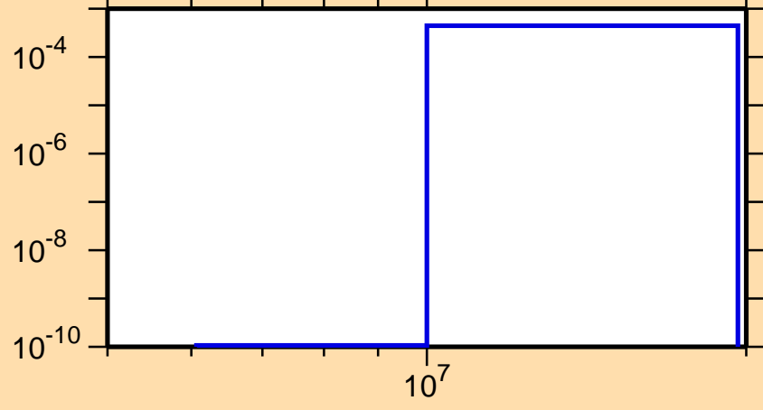
\sigma vs. E for ^{166}\text{Ho}(n,np)
