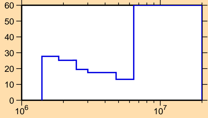
\Delta\sigma/\sigma vs. E for ^{166}\text{Ho}(n,ncont.)
