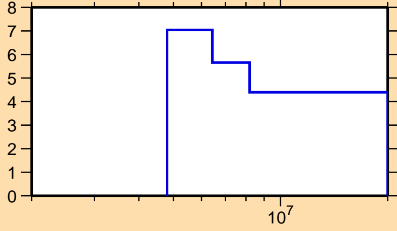
\Delta\sigma/\sigma vs. E for ^{166}\text{Ho}(n,\text{nonel.})
