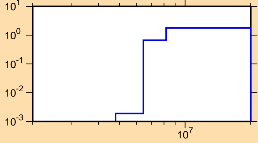
\sigma vs. E for ^{166}\text{Ho}(n,2n)
