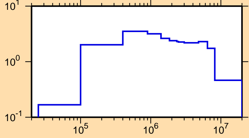
\sigma vs. E for ^{166}\text{Ho}(n,\text{inel.})
