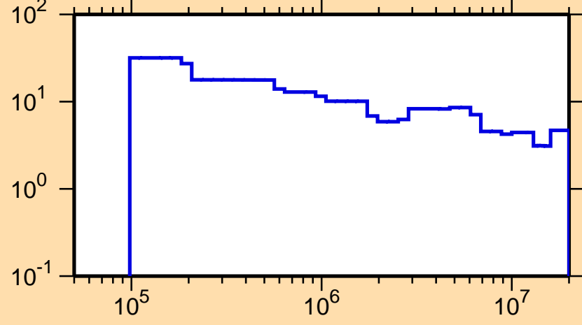
\Delta\sigma/\sigma vs. E for ^{167}\text{Ho}(n,\text{tot.})
