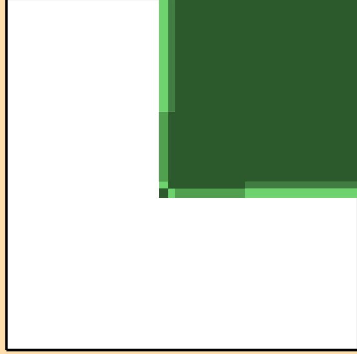
\sigma vs. E for ^{167}\text{Ho}(n,3n)
