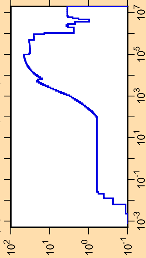
\Delta\mu/\mu vs. E for ^{168}\text{Ho}(\text{mt251})
