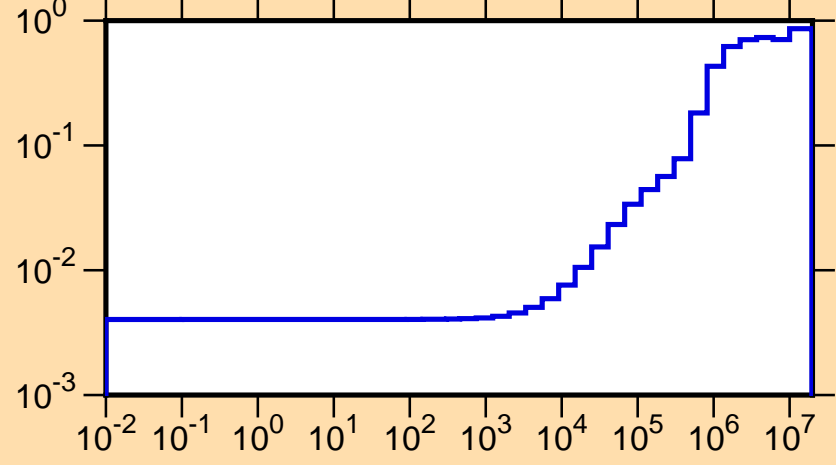
\mu vs. E for ^{168}\text{Ho}(\text{mt251})
