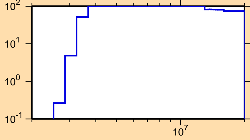
\Delta\sigma/\sigma vs. E for ^{168}\text{Ho}(n,p)
