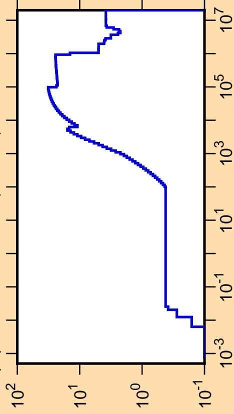
\Delta\mu/\mu vs. E for ^{169}\text{Ho}(\text{mt251})
