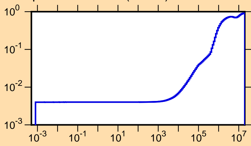
\mu vs. E for ^{169}\text{Ho}(\text{mt251})
