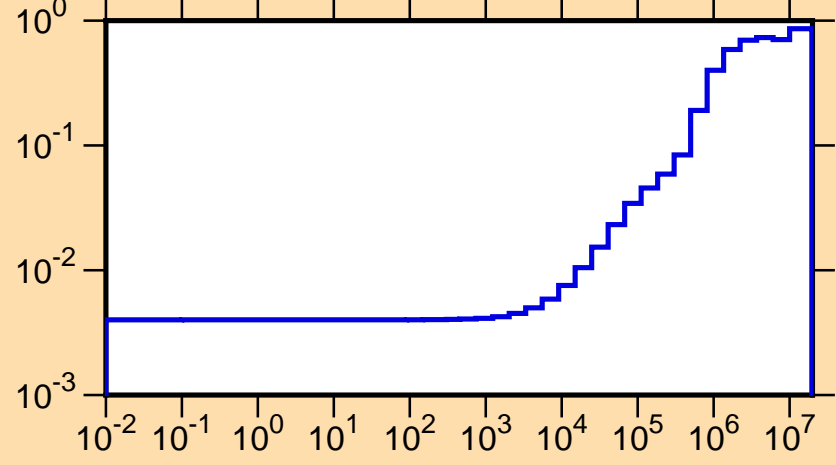
\mu vs. E for ^{169}\text{Ho}(\text{mt251})
