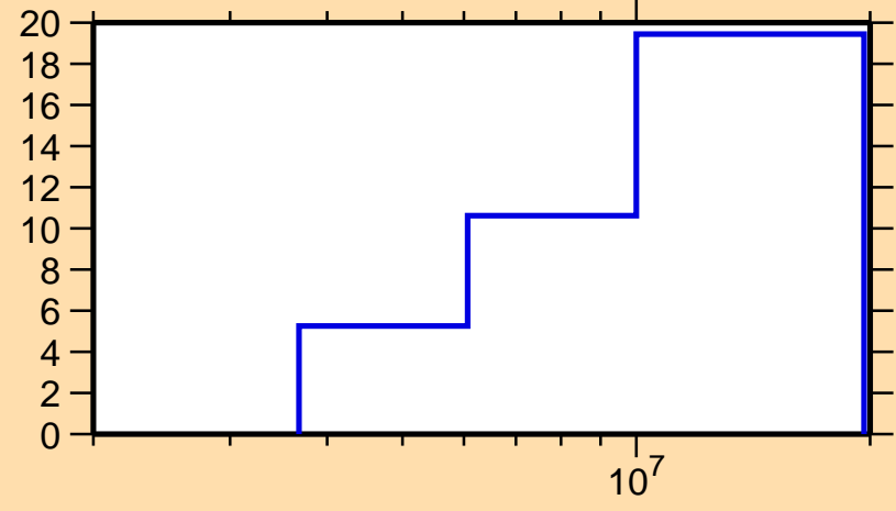
\Delta\sigma/\sigma vs. E for ^{169}\text{Ho}(n,ncont.)
