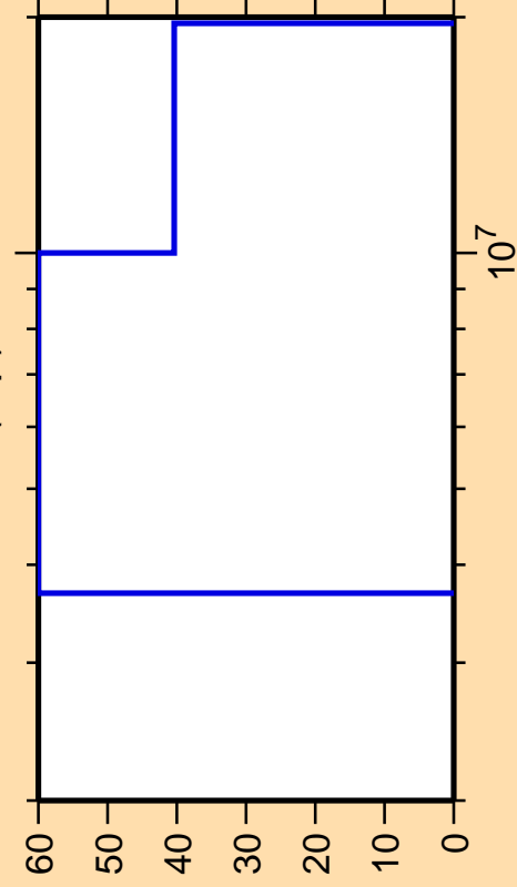
\Delta\sigma/\sigma vs. E for ^{169}\text{Ho}(n,p)
