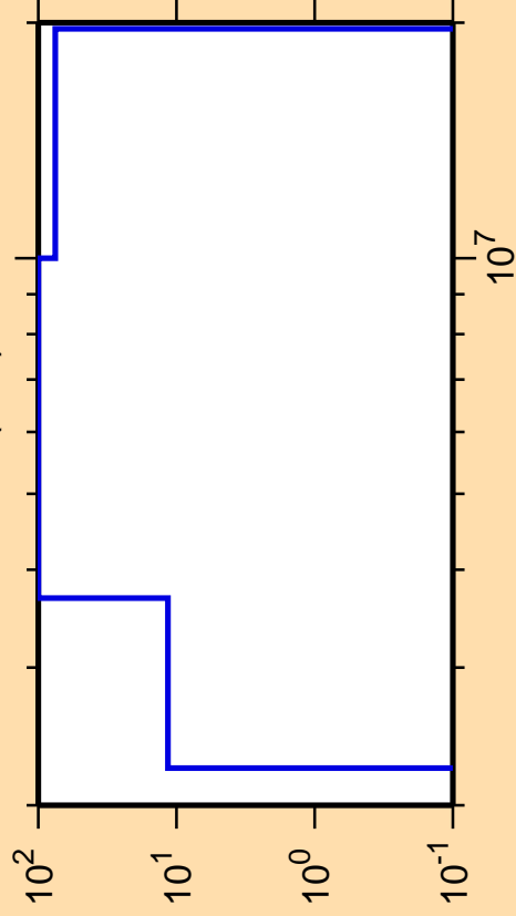
\Delta\sigma/\sigma vs. E for ^{169}\text{Ho}(n,\alpha)
