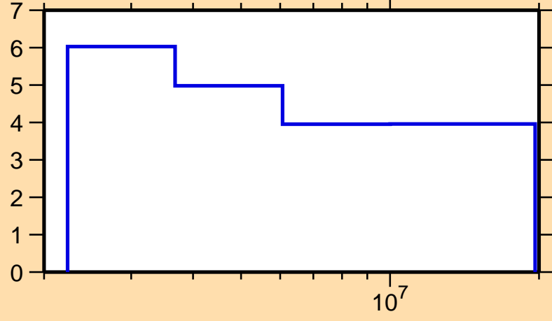
\Delta\sigma/\sigma vs. E for ^{169}\text{Ho}(n,\text{nonel.})
