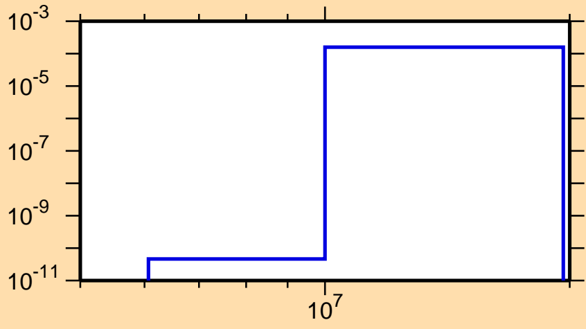
\sigma vs. E for ^{169}\text{Ho}(n,d)
