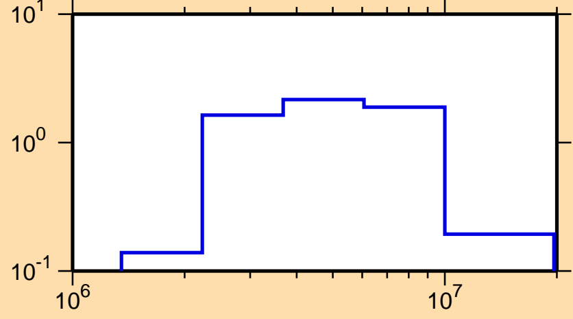
\sigma vs. E for ^{169}\text{Ho}(n,n\text{cont.})
