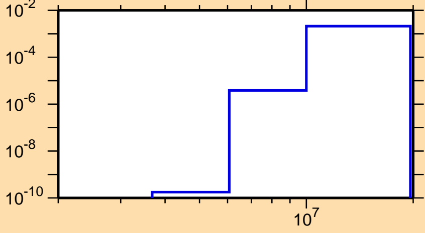
\sigma vs. E for ^{169}\text{Ho}(n,p)
