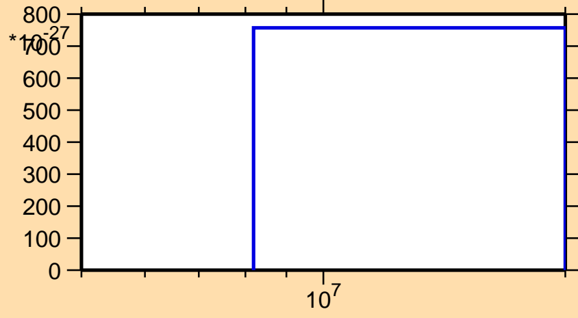
\sigma vs. E for ^{169}\text{Ho} (mt 42)
