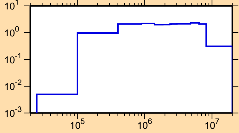
\sigma vs. E for ^{169}\text{Ho}(n,\text{inel.})
