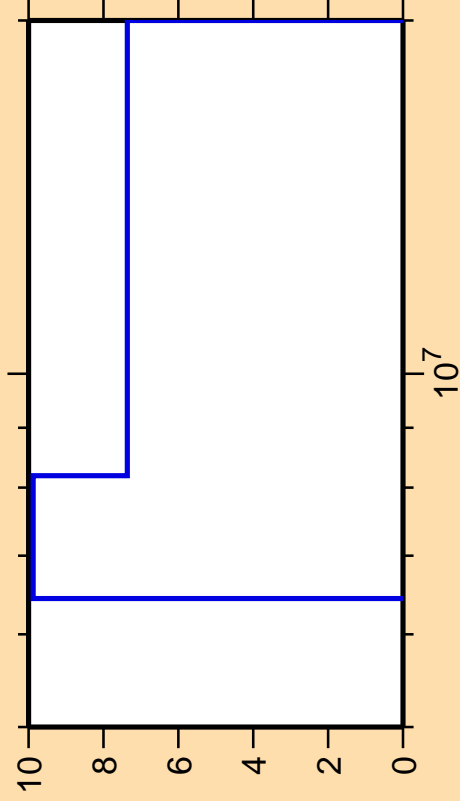
\Delta\sigma/\sigma vs. E for ^{169}\text{Ho}(n,2n)
