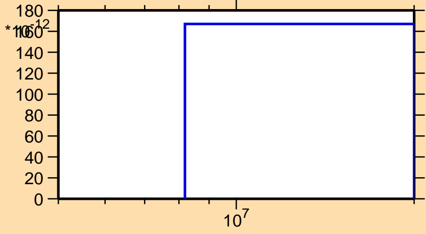
\sigma vs. E for ^{169}\text{Ho}(n,2n\alpha)
