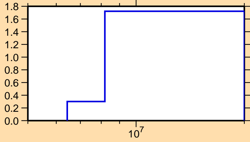
\sigma vs. E for ^{169}\text{Ho}(n,2n)
