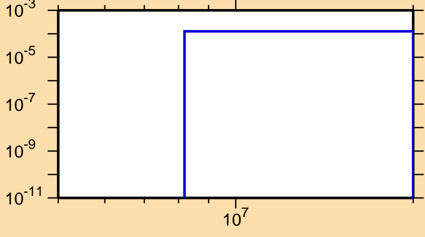
\sigma vs. E for ^{169}\text{Ho}(n,d)
