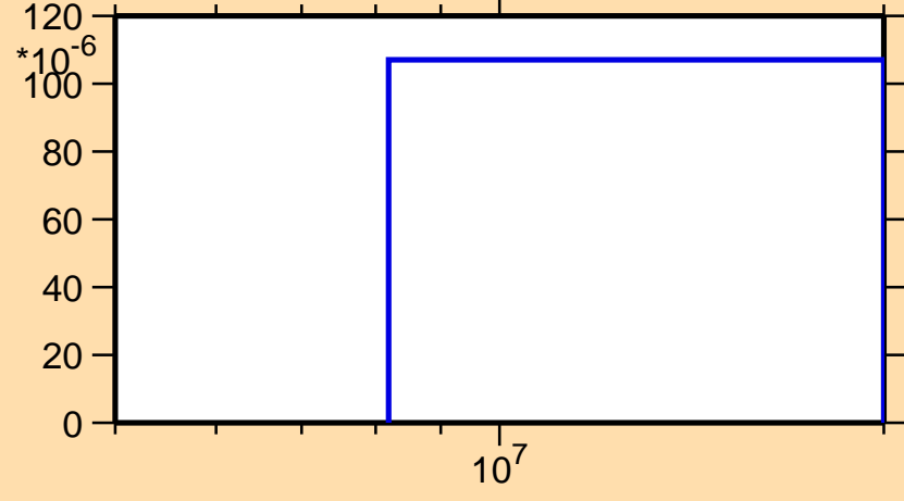
\sigma vs. E for ^{169}\text{Ho}(n,np)
