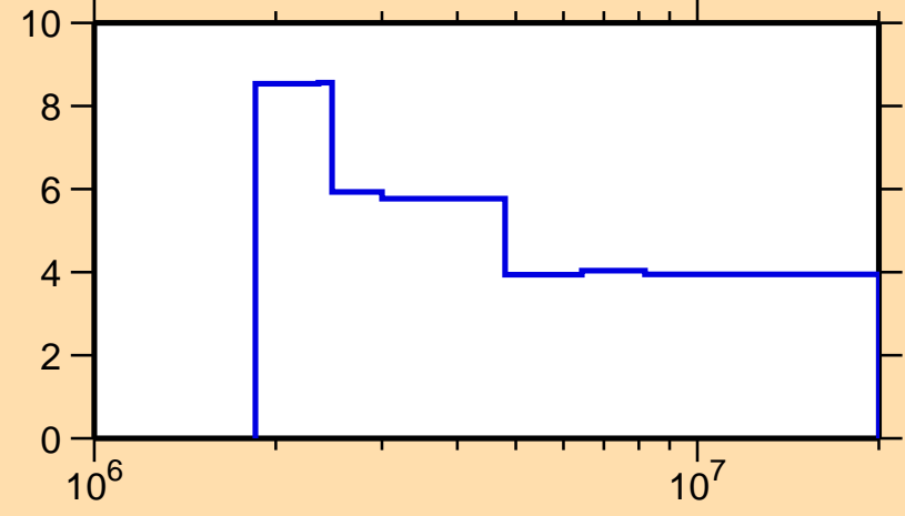
\Delta\sigma/\sigma vs. E for ^{169}\text{Ho}(n,n\text{onel.})
