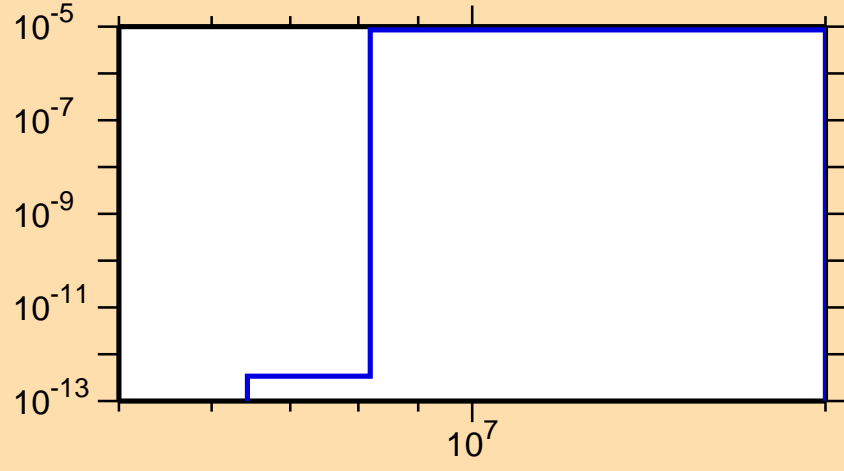
\sigma vs. E for ^{169}\text{Ho}(n,n\alpha)
