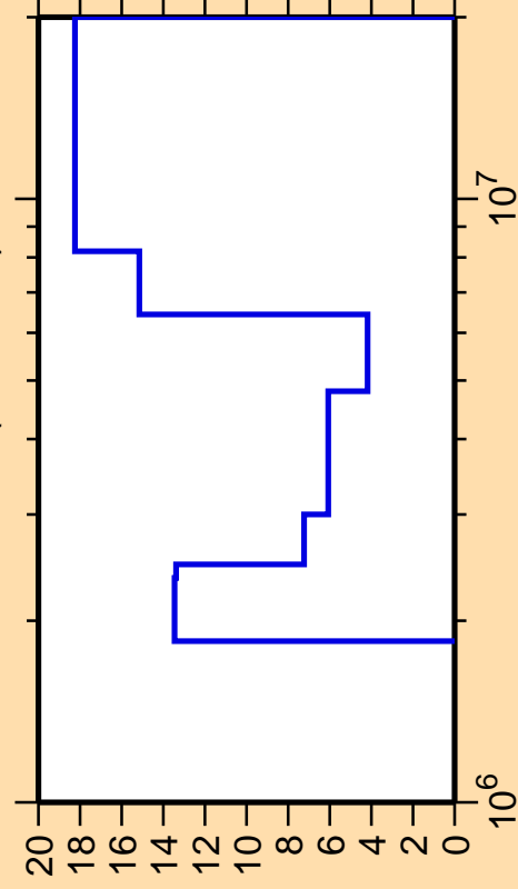
\Delta\sigma/\sigma vs. E for ^{169}\text{Ho}(n,\text{ncont.})
