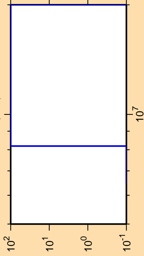
\Delta\sigma/\sigma vs. E for ^{169}\text{Ho}(n,d)
