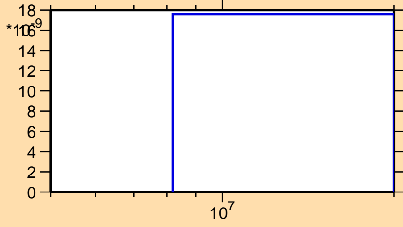
\sigma vs. E for ^{169}\text{Ho}(n,\text{nt})
