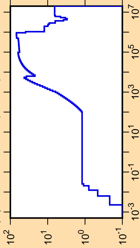
\Delta\mu/\mu vs. E for ^{170}\text{Ho}(\text{mt251})
