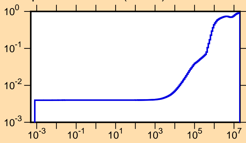
\mu vs. E for ^{170}\text{Ho}(\text{mt251})
